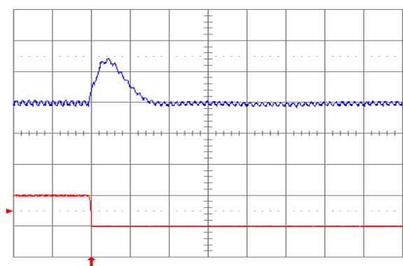
Fig. 2.0V.8: Output voltage response (YNL05S10020) to negative load current step change from 10 A to 5 A with slew rate of -5 A/ \mu\text{s} at V_{in} = 5\text{ V} . Top trace: output voltage (100 mV/div.); Bottom trace: load current (5 A/div.). C_o = 47\ \mu\text{F} ceramic + 1 \mu\text{F} ceramic. Time scale: 20 \mu\text{s} /div.
