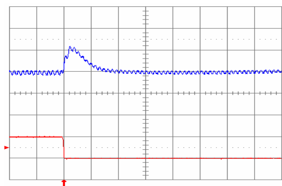
Fig. 2.5V.8: Output voltage response (YNL05S10025) to negative load current step change from 10 A to 5 A with slew rate of -5 A/ \mu\text{s} at V_{in} = 5\text{ V} . Top trace: output voltage (100 mV/div.); Bottom trace: load current (5 A/div.). C_o = 47\text{ }\mu\text{F} ceramic + 1 \mu\text{F} ceramic. Time scale: 20 \mu\text{s} /div.
