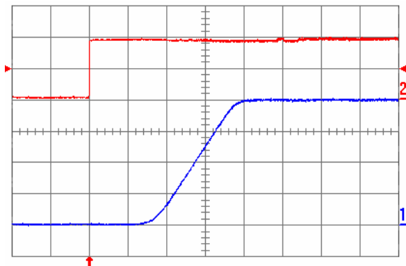
Fig. 2.0V.5: Turn-on transient (YNL05S10020) with the application of Enable signal at full rated load current (resistive) and 47 \mu\text{F} external capacitance at V_{in} = 5\text{ V} . Top trace: Enable signal (2 V/div.); Bottom trace: output voltage (500 mV/div.); Time scale: 2 ms/div.
