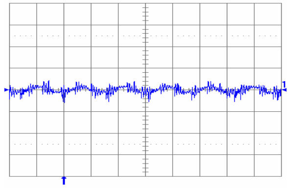
Fig. 1.5V.6: Output voltage ripple (20 mV/div.) at full rated load current into a resistive load with external capacitance 47 \mu\text{F} ceramic + 1 \mu\text{F} ceramic and V_{in} = 5\text{ V} (YNL05S10015). Time scale: 2 \mu\text{s} /div.
