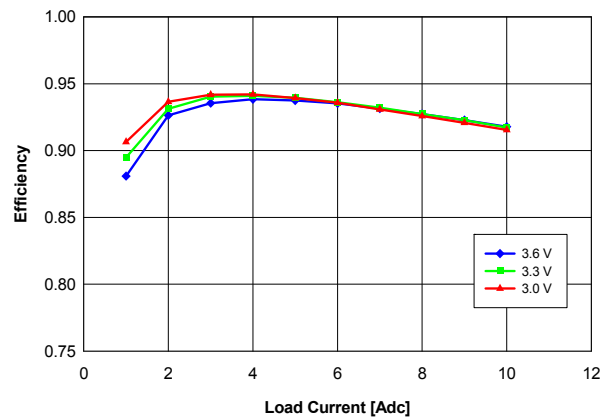
Fig. 1.8V.4: Efficiency vs. load current and input voltage for YNL05S10018 converter mounted horizontally with air flowing at a rate of 200 LFM (1 m/s) and T_a = 25\text{ }^{\circ}\text{C} .
