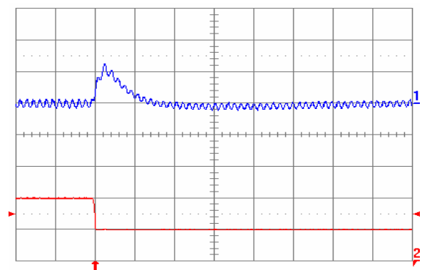
Fig. 3.3V.8: Output voltage response (YNL05S10033) to negative load current step change from 10 A to 5 A with slew rate of -5 A/ \mu\text{s} at V_{\text{in}} = 5\text{ V} . Top trace: output voltage (100 mV/div.); Bottom trace: load current (5 A/div.). C_{\text{o}} = 47\text{ }\mu\text{F} ceramic + 1 \mu\text{F} ceramic. Time scale: 20 \mu\text{s} /div.
