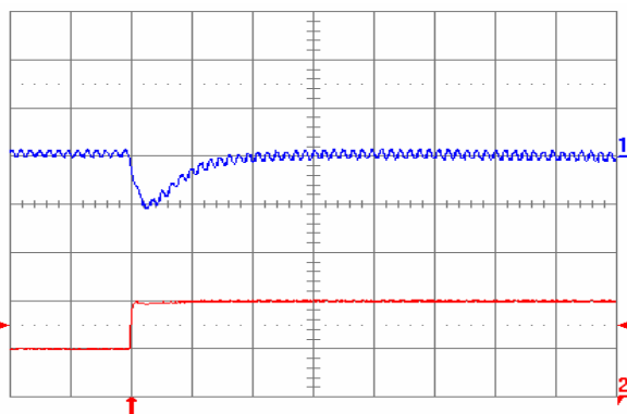
Fig. 2.5V.7: Output voltage response (YNL05S10025) to positive load current step change from 5 A to 10 A with slew rate of 5 A/ \mu\text{s} at V_{in} = 5\text{ V} . Top trace: output voltage (100 mV/div.); Bottom trace: load current (5 A/div.). C_o = 47\text{ }\mu\text{F} ceramic + 1 \mu\text{F} ceramic. Time scale: 20 \mu\text{s} /div.
