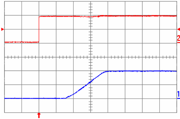
Fig. 1.0V.5: Turn-on transient (YNL05S10010) with the application of Enable signal at full rated load current (resistive) and 47 \mu\text{F} external capacitance at V_{in} = 5\text{ V} . Top trace: Enable signal (2 V/div.); Bottom trace: output voltage (500 mV/div.); Time scale: 2 ms/div.
