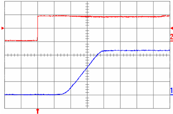
Fig. 3.3V.5: Turn-on transient (YNL05S10033) with the application of Enable signal at full rated load current (resistive) and 47 \mu\text{F} external capacitance at V_{\text{in}} = 5\text{ V} . Top trace: Enable signal (2 V/div.); Bottom trace: output voltage (1 V/div.); Time scale: 2 ms/div.
