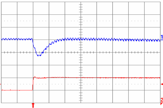
Fig. 1.2V.6: Output voltage response (YNL05S10012) to positive load current step change from 5 A to 10 A with slew rate of 5 A/ \mu\text{s} at V_{in} = 5\text{ V} . Top trace: output voltage (100 mV/div.); Bottom trace: load current (5 A/div.). C_o = 47\ \mu\text{F} ceramic + 1 \mu\text{F} ceramic. Time scale: 20 \mu\text{s} /div.
