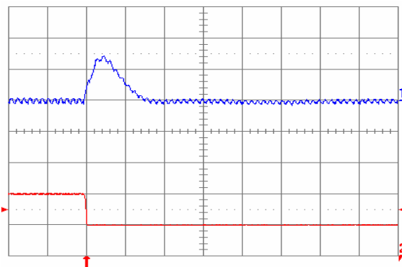
Fig. 1.8V.8: Output voltage response (YNL05S10018) to negative load current step change from 10 A to 5 A with slew rate of -5 A/ \mu s at V_{in} = 5 V. Top trace: output voltage (100 mV/div.); Bottom trace: load current (5 A/div.). C_o = 47 \mu F ceramic + 1 \mu F ceramic. Time scale: 20 \mu s/div.
