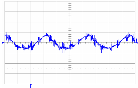
Fig. 3.3V.6: Output voltage ripple (20 mV/div.) at full rated load current into a resistive load with external capacitance 47 \mu\text{F} ceramic + 1 \mu\text{F} ceramic and V_{\text{in}} = 5\text{ V} (YNL05S10033). Time scale: 2 \mu\text{s} /div.
