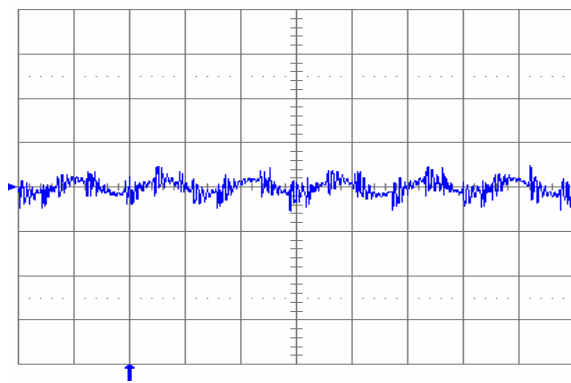
Fig. 2.0V.6: Output voltage ripple (20 mV/div.) at full rated load current into a resistive load with external capacitance 47 \mu\text{F} ceramic + 1 \mu\text{F} ceramic and V_{in} = 5\text{ V} (YNL05S10020). Time scale: 2 \mu\text{s} /div.
