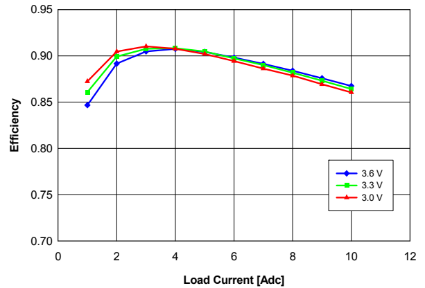
Fig. 1.0V.4: Efficiency vs. load current and input voltage for YNL05S10010 converter mounted horizontally with air flowing at a rate of 200 LFM (1 m/s) and T_a = 25\text{ }^\circ\text{C} .
