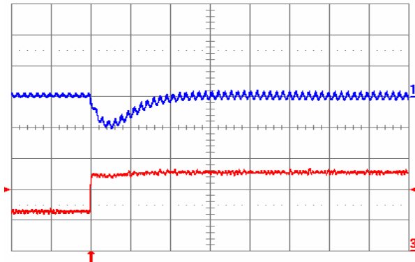
Fig. 1.0V.7: Output voltage response (YNL05S10010) to positive load current step change from 5 A to 10 A with slew rate of 5 A/ \mu\text{s} at V_{in} = 5\text{ V} . Top trace: output voltage (100 mV/div.); Bottom trace: load current (5 A/div.). C_o = 47\ \mu\text{F} ceramic + 1 \mu\text{F} ceramic. Time scale: 20 \mu\text{s} /div.
