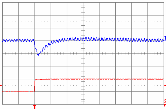
Fig. 3.3V.7: Output voltage (YNL05S10033) to positive load current step change from 5 A to 10 A with slew rate of 5 A/ \mu\text{s} at V_{\text{in}} = 5\text{ V} . Top trace: output voltage (100 mV/div.); Bottom trace: load current (5 A/div.). C_{\text{o}} = 47\text{ }\mu\text{F} ceramic + 1 \mu\text{F} ceramic. Time scale: 20 \mu\text{s} /div.
