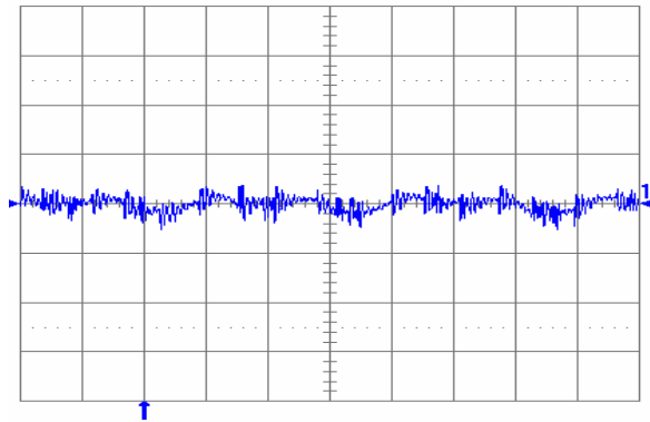
Fig. 1.0V.6: Output voltage ripple (20 mV/div.) at full rated load current into a resistive load with external capacitance 47 \mu\text{F} ceramic + 1 \mu\text{F} ceramic and V_{in} = 5\text{ V} (YNL05S10010). Time scale: 2 \mu\text{s} /div.
