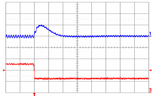
Fig. 1.0V.8: Output voltage response (YNL05S10010) to negative load current step change from 10 A to 5 A with slew rate of -5 A/ \mu\text{s} at V_{in} = 5\text{ V} . Top trace: output voltage (100 mV/div.); Bottom trace: load current (5 A/div.). C_o = 47\ \mu\text{F} ceramic + 1 \mu\text{F} ceramic. Time scale: 20 \mu\text{s} /div.
